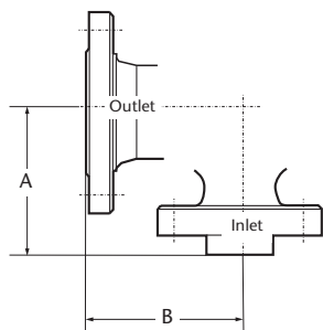
Nominal inlet diameter <4" A and B ± 1.6 mm Nominal outlet diameter >4" A and B ± 3.2 mm
