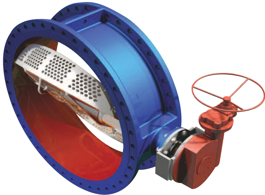
Butterfly valve with anti-cavitation cowel
